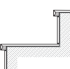
DETALLE / DETAIL
